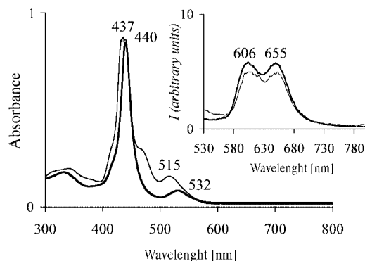
Figure 4. Normalised absorption and emission spectra (inset) of an optically matched solution of 5 (thin) and 7 -PF 6 (bold) (excitation at 438 nm) at 298 K in dichloromethane.
