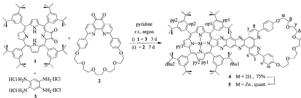
Figure 1. Stepwise condensation of the two diones with the bridging spacer.
