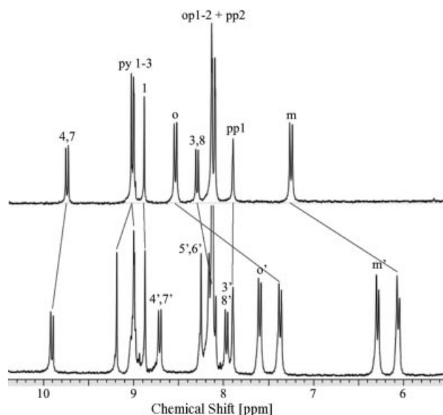
Figure 2. ^1\text{H} NMR spectra (aromatic region) of compounds 5 and 7 · \text{PF}_6^- in \text{CD}_2\text{Cl}_2 .
