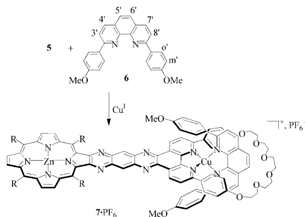
Figure 3. The threading reaction affording pseudorotaxane 7 .
